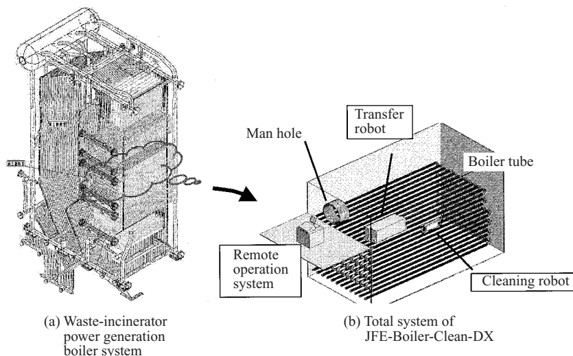
Fig. 1 System of JFE-Boiler-Clean-DX
