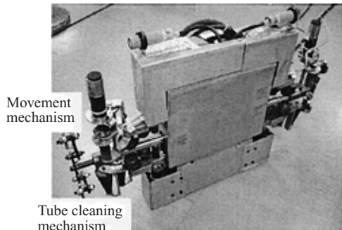
Photo 2 Outlook of JFE-Boiler-Clean-DX
