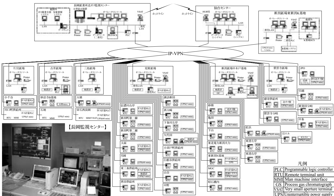
Fig.1 Nagaoka SCADA network
