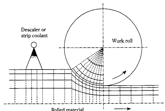
Fig. 3 Schematic diagram of elemental division during rolling
