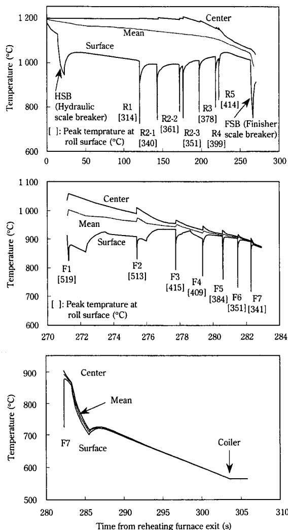
Fig. 9 Temperature changes at leading end of rolled material from exit of reheating furnace to coiler
