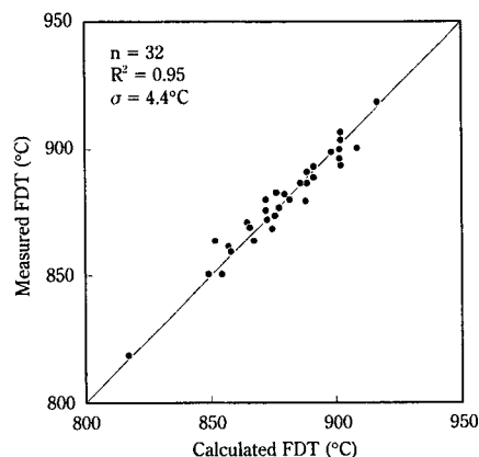
Fig. 6 Comparison between calculated and measured finisher delivery temperatures
