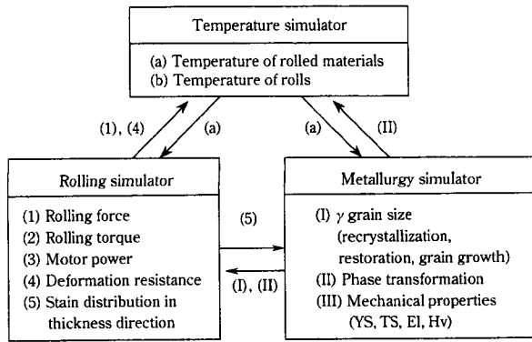
Fig. 1 Interrelation among various simulators
