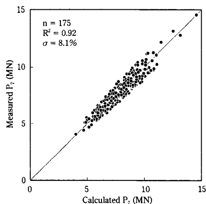
Fig. 7 Comparison between calculated and measured rolling forces at F7 stand
