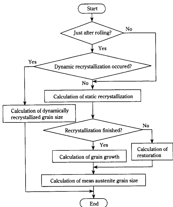
Fig. 4 Flow chart for calculating \gamma grain size
