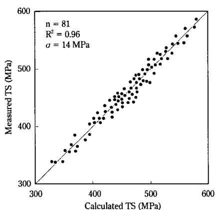
Fig. 8 Comparison between calculated and measured tensile strength of final product
