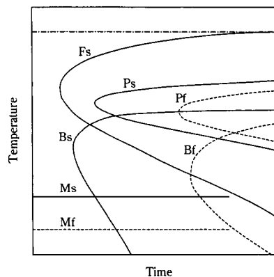
Fig. 5 Schematic TTT diagrams; F, P, B and M represent ferrite, pearlite, bainite and martensite, respectively, and subscripts s and f represent start and finish of phase transformation, respectively
