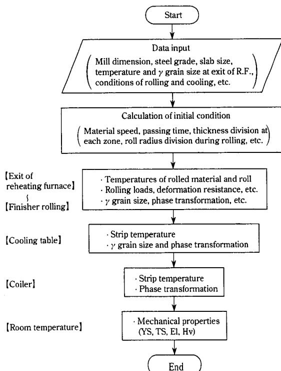
Fig. 2 Whole simulation flow of the hot integrated mathematical simulator
