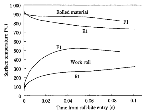
Fig. 10 Surface temperature changes in roll bites during R1 and F1 rollings at leading end of rolled material
