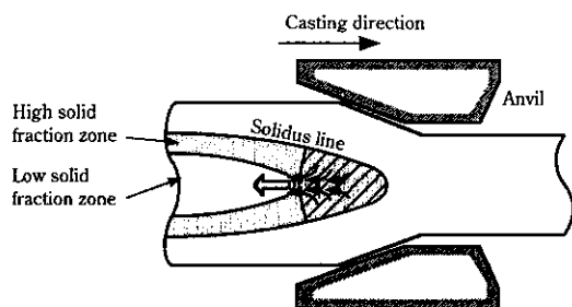
Fig. 8 Concept of continuous forging process
