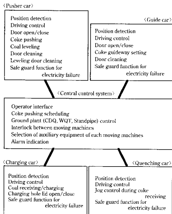
Fig. 3 Functional workshare of the automatic control system
