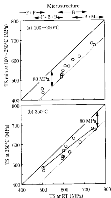
Fig. 2 Relationship between tensile strength at RT and that at elevated temperatures
