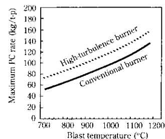
Fig. 13 Comparison of PC rate between conventional and high-turbulence burner
