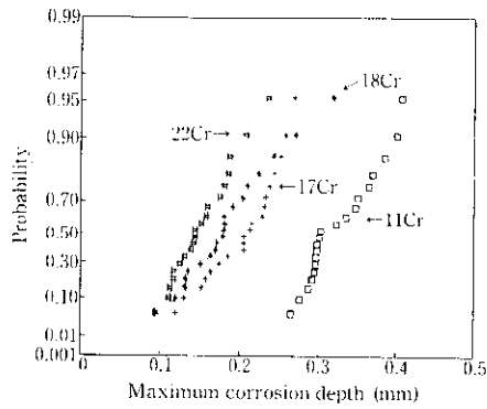
Fig. 3 Doubly exponential probability plots of the maximum corrosion depth of Fe-Cr steels after the synthetic condensate corrosion test
