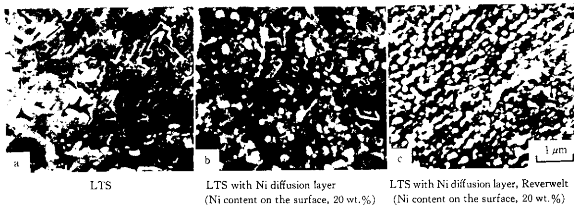
Photo 2 Scanning electro micrographs of alloy layer (stripped side surface) at an interface of alloy and base steel
