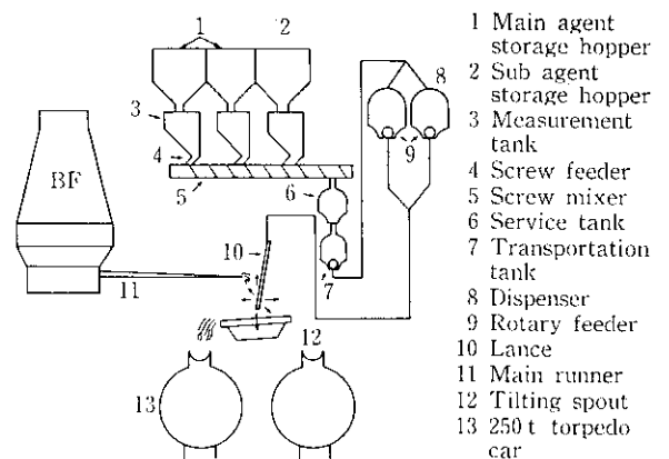
Fig. 3 Outline of desilicization equipment 1)
