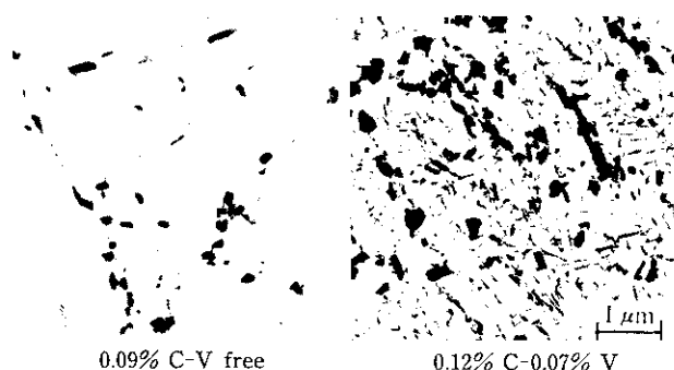
Photo 2 Extraction replica microstructures of single pass weld metal after PWHT of 690 °C x 12 h
