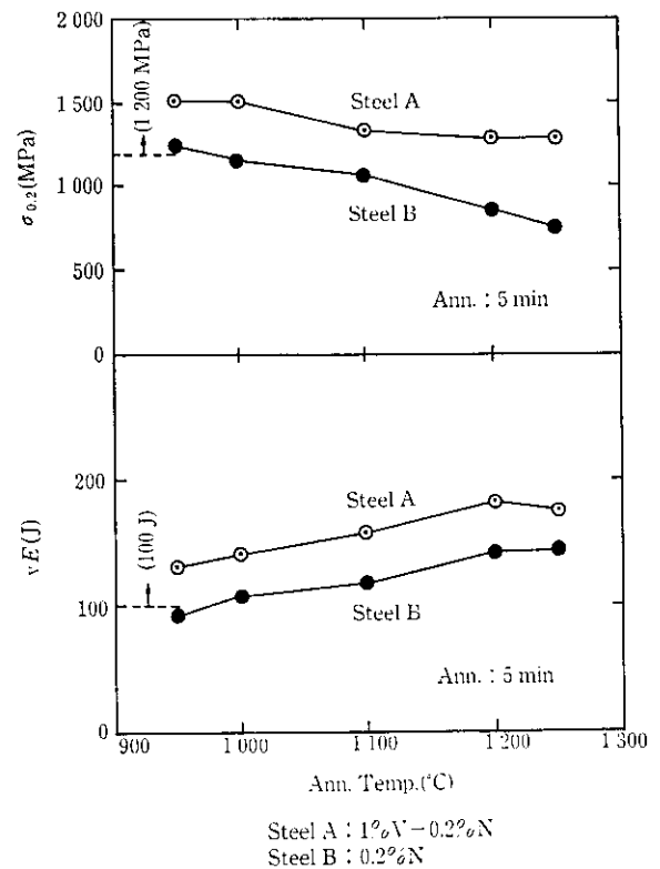
Fig. 7 Change in \sigma_{0.2} and vE at 4 \text{ K} with annealing (solution heat treatment) temperature
