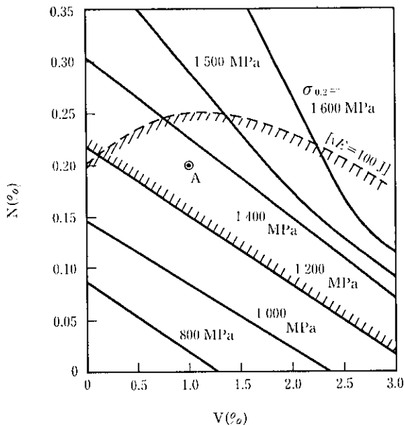
Fig. 5 Equivalent curves of \sigma_{0.2} of annealed materials ( 1100^{\circ}\text{C} \times 5 \text{ min} ) at 4 \text{ K} with vanadium and nitrogen contents as variables
