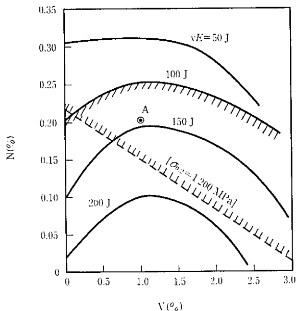
Fig. 6 Equivalent curves of vE of annealed materials ( 1100^{\circ}\text{C} \times 5 \text{ min} ) at 4 \text{ K} with vanadium and nitrogen contents as variables
