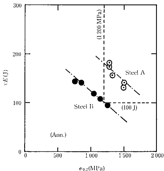
Fig. 9 Relation between \sigma_{0.2} and \nu E at 4 K of steel A and steel B (Area given by the condition, \sigma_{0.2} \geq 1200 MPa and \nu E \geq 100 J, is proposed by JAERI for fusion furnace superconducting magnet.)
