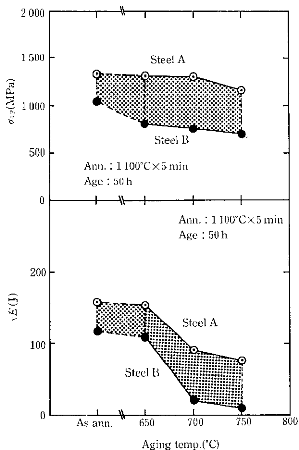
Fig. 10 Change in \sigma_{0.2} and \nu E at 4 K with aging ( \text{Nb}_3\text{Sn} precipitation heat treatment) temperature, where specimens were annealed and then aged
