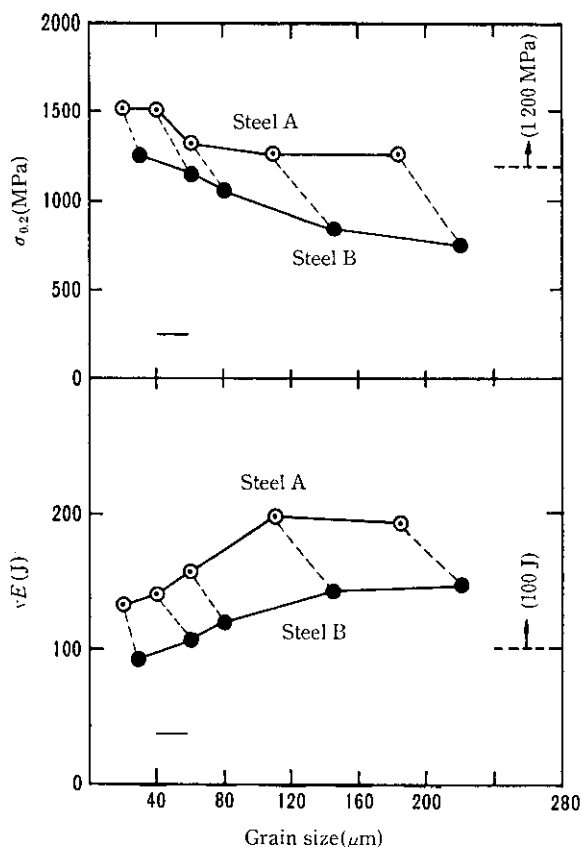
Fig. 8 Change in \sigma_{0.2} and \nu E at 4 K with grain size
