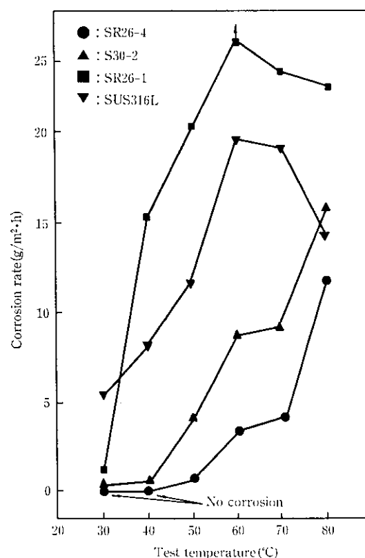
Fig. 11 Corrosion rate in 10% FeCl 3 ·6H 2 O solution for 45 h (the specimens were tied with glass rods by rubber bands.)
