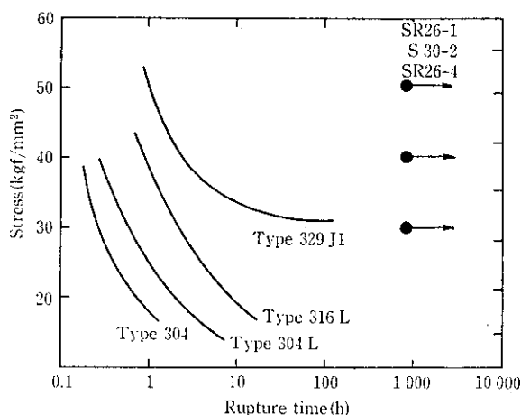
Fig. 13 Resistance to stress corrosion cracking of stainless steels uniaxially stressed in boiling 42% \text{MgCl}_2 solution
