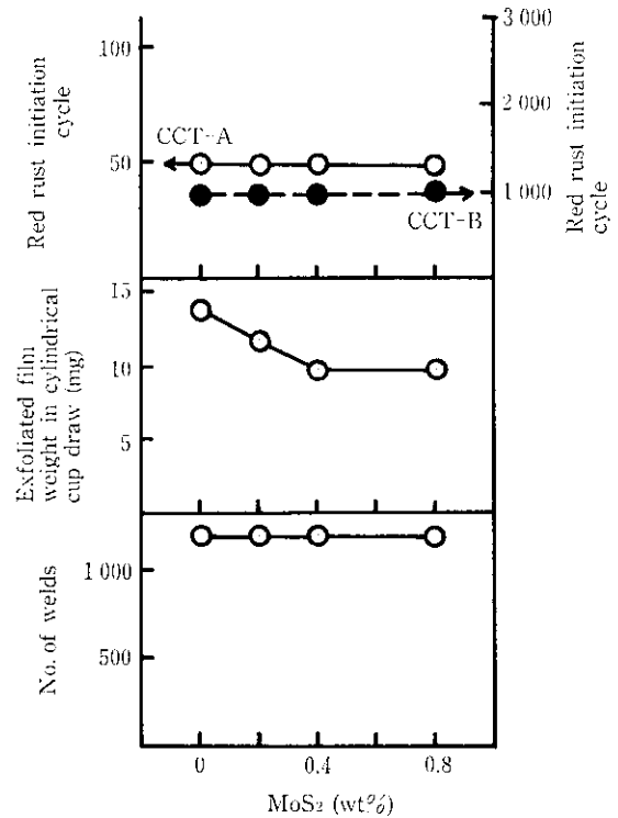
Fig. 5 Effect of MoS 2 addition to zinc rich film on (a) weldability, (b) coating adhesion and (c) corrosion resistance
