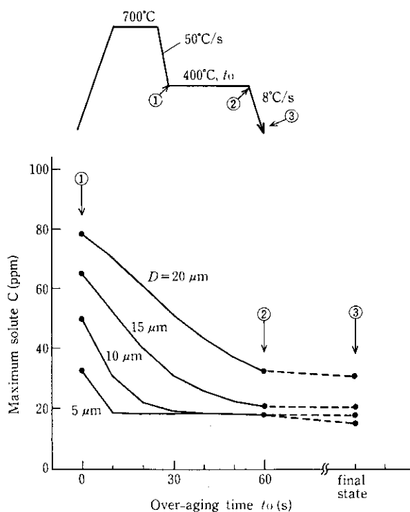
Fig. 16 Effects of ferrite grain diameter D and over-aging time on the decrease in the maximum solute carbon content
