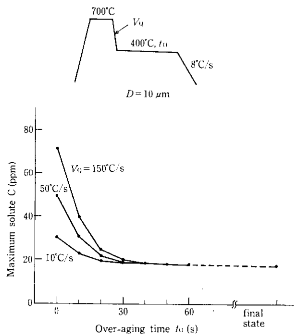
Fig. 17 Effect of the cooling rate on the decrease in the maximum solute carbon content
