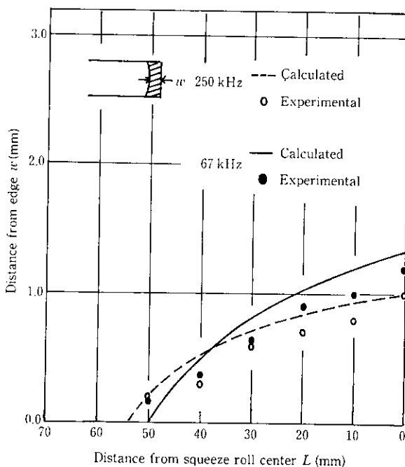
Fig. 6 Change in area of heated zone
