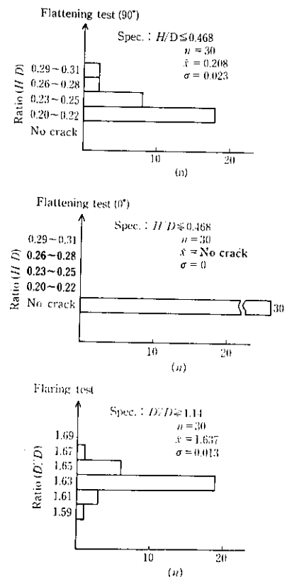
Fig. 7 Flattening and flaring test (STBA 22E-G 48.6 φ × 4.2 t)
