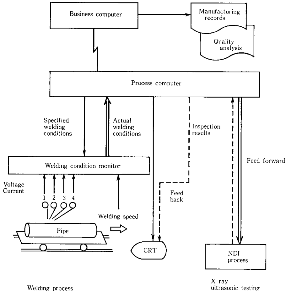
Fig. 5 Quality control for welding process
