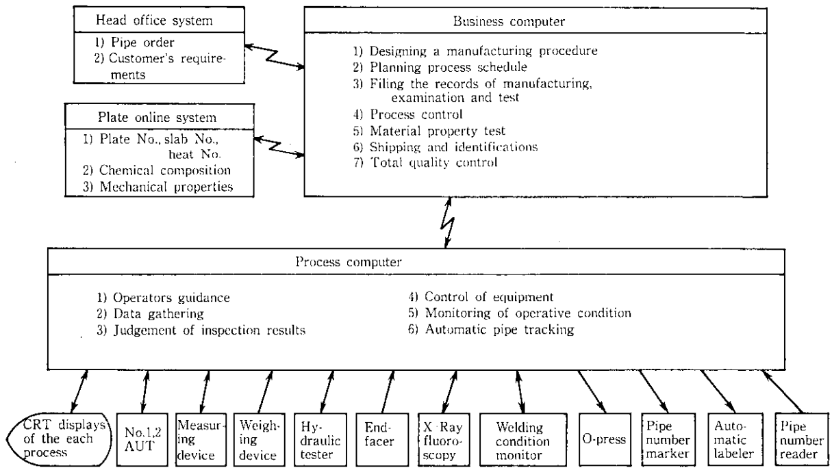
Fig. 2 System construction
