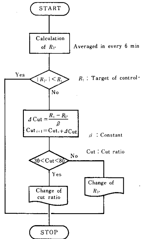
Fig. 9 Flow chart for the permeability control system
