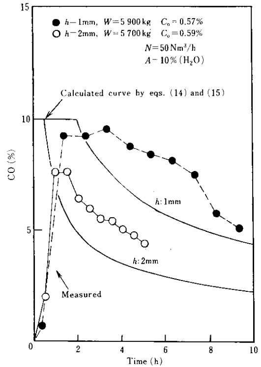
Fig. 2 Transition of CO (%) during open coil annealing
