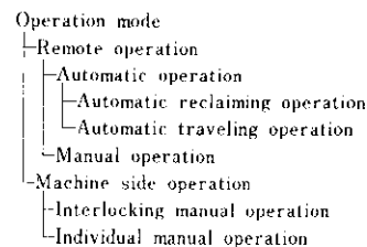
Fig.3 Operation mode of reclaimer
