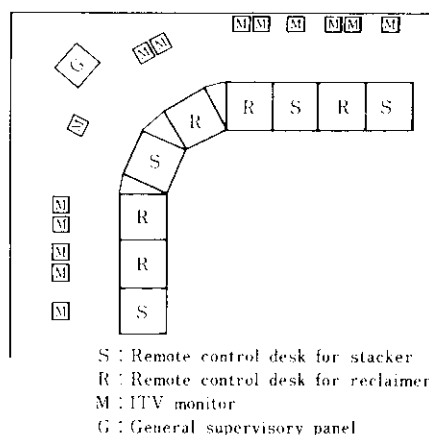
Fig. 5 Layout of operation room
