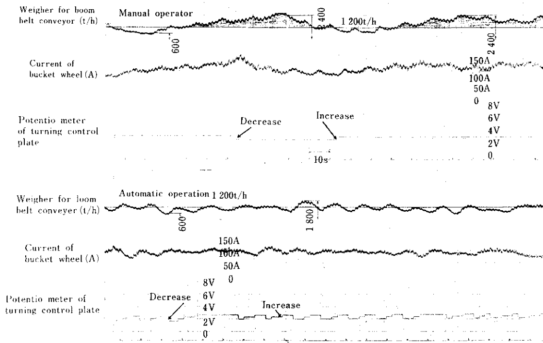
Fig. 9 Reclaiming chart of reclaimer
