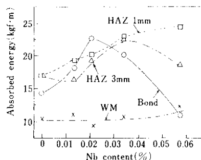
Fig. 5 Effect of Nb content on absorbed energy at -51°C of submerged arc welded joint of controlled rolled and normalized plates
