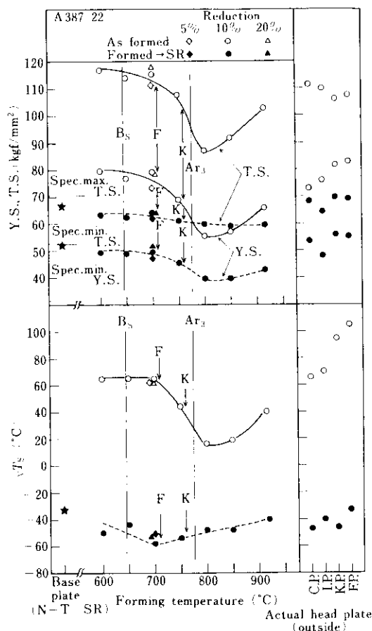
Fig.21 Mechanical properties of the A387-22 steel specimens simulated to the hot press forming process as a function of forming temperature (heating temp.: 925°C)
