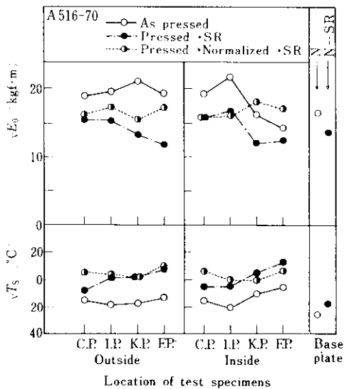
Fig.9 Charpy impact properties of the A516-70 steel head plate by the hot press forming process
