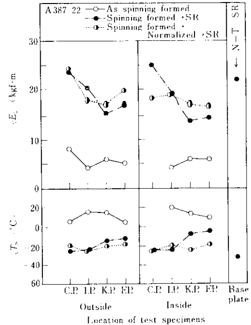
Fig. 19 Charpy impact properties of the A387-22 steel head plate formed by the hot spinning forming process
