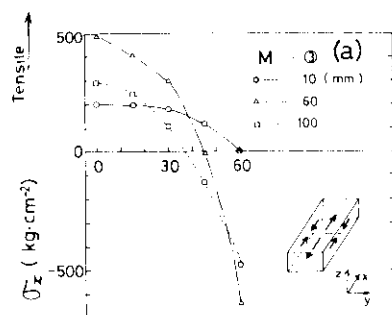
Fig. 4 Thermal stresses produced in refractory during heating from one end
