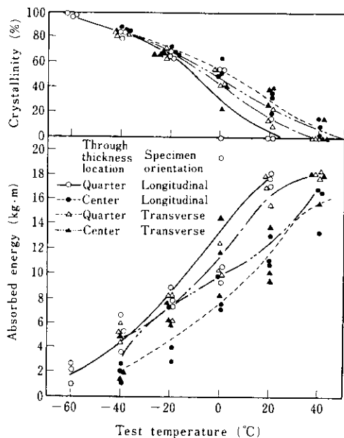
Fig. 3 Results of 2mm V-notch Charpy impact tests
