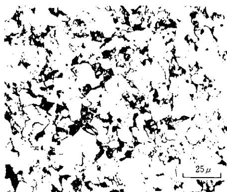
Photo. 1 Optical micrograph of normalized and tempered steel at the center of 75mm thick plate
