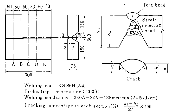
Fig. 13 Specimen for reheat cracking test
