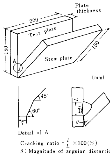
Fig. 1 Specimen of Cranfield test
