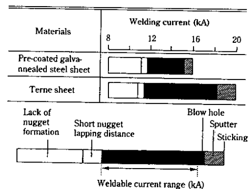
Fig. 3 Comparison of weldable current range on seam welding
