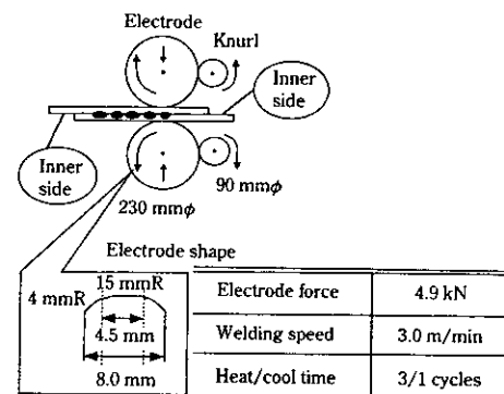
Fig. 2 Seam welding conditions
