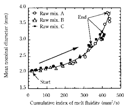
Fig. 6 Relationship between cumulative index of melt fluidity and mean nominal diameter of grain through sintering process
