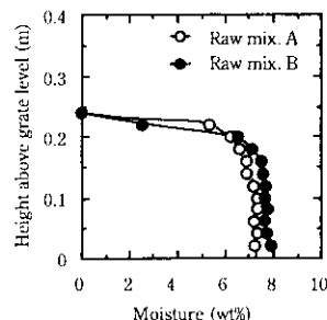
Fig. 8 Moisture condensation in sintering bed with blending of pisolitic ore
