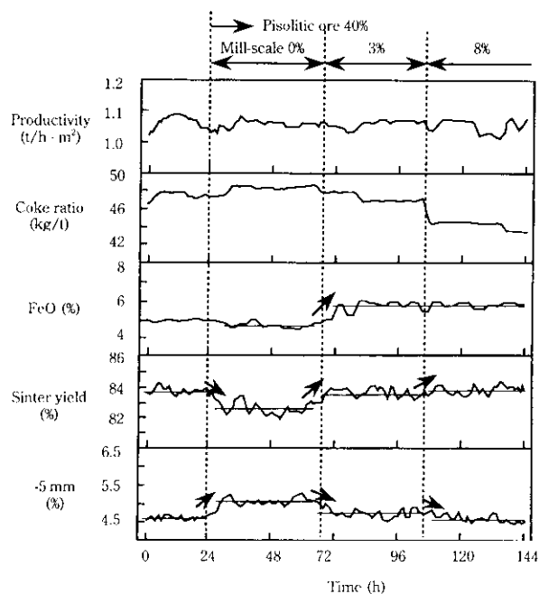
Fig. 14 Operation results using mill-scale with a large amount of pisolitic ore
