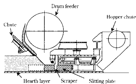
Fig. 15 Outline of the poromeric improvement machine
