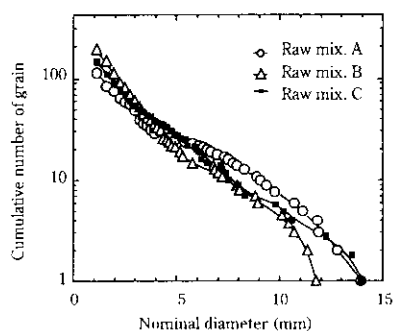
Fig. 5 Grain size distribution of sinter cake with blending of pisolitic ore and mill-scale
