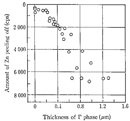
Fig. 14 Influence of thickness of \Gamma phase on powdering property
