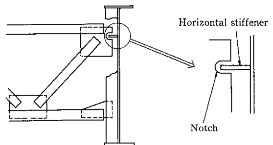
Fig. 6 Gusset plate with automatically drawn notch
