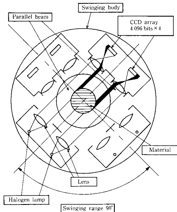
Fig. 8 Principle of profile meter
