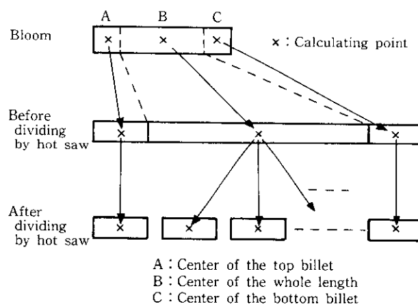
Fig. 9 Evaluation of the temperature of bloom at different three points
