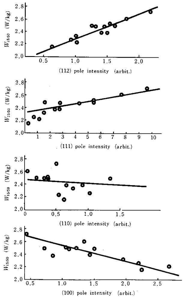
Fig. 4 Relationship between pole intensity and core loss ( W_{15/50}, 0.50\text{ mm} )
