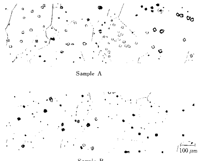
Photo. 5 Facet pit of the specimen surface
