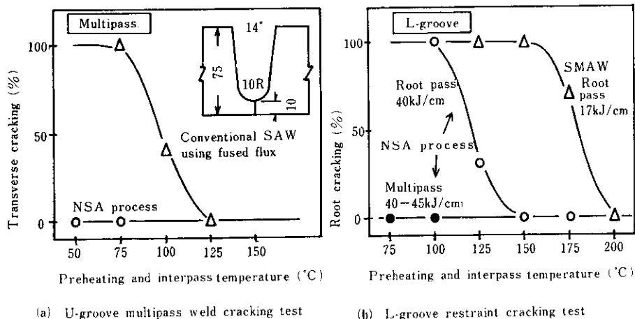
Fig. 9 Restraint weld cracking test results of NSA welding materials for ASTM A387 Gr.22 steel (Test procedure: WES 3005)
