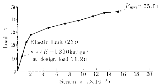
Fig. 12 Load-strain curve at loading position ② (strain gauge 8) of Type-2A ( \sigma : stress, E : Elastic modulus)
